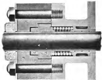
Fig. 1016. Jerome Metallic Rod Packing. Jerome & Elliot.
